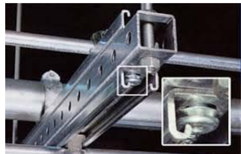
Structural Ceiling Grid System
